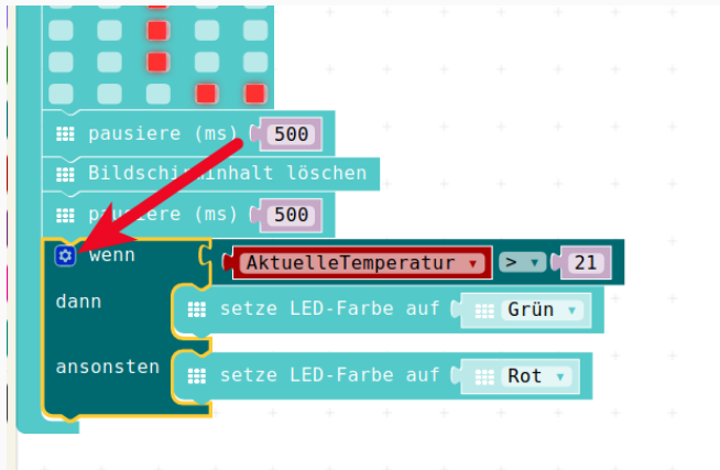
Figure 2: ToolBox
