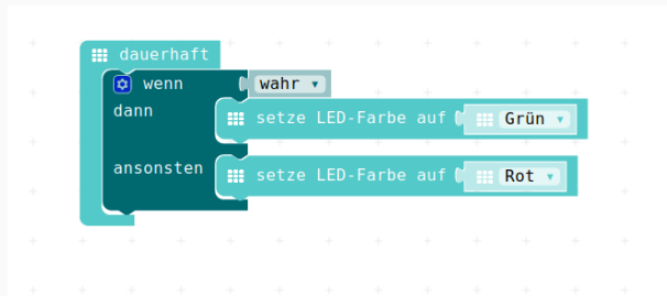
Figure 8: RGB Led In Wenn Wahr
